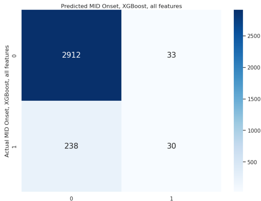
Figure 4-3. Confusion matrix all features, XGBoost - onset
